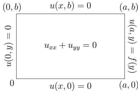
FIGURE 1. Laplace Equation with Dirichlet Boundary Condition (4).
