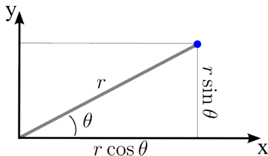
Figure 1. Polar coordinates
