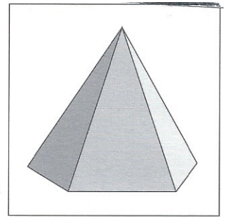
Pentagonal Pyramid
