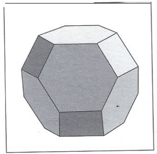
Truncated Octahedron
