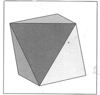
Octahedron
