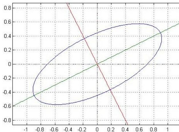
Figure 2.1: 2x^2 - 4xy + 5y^2 = 1 , the ellipse x^2 + 6y^2 = 1 rotated through \pi/6 .
