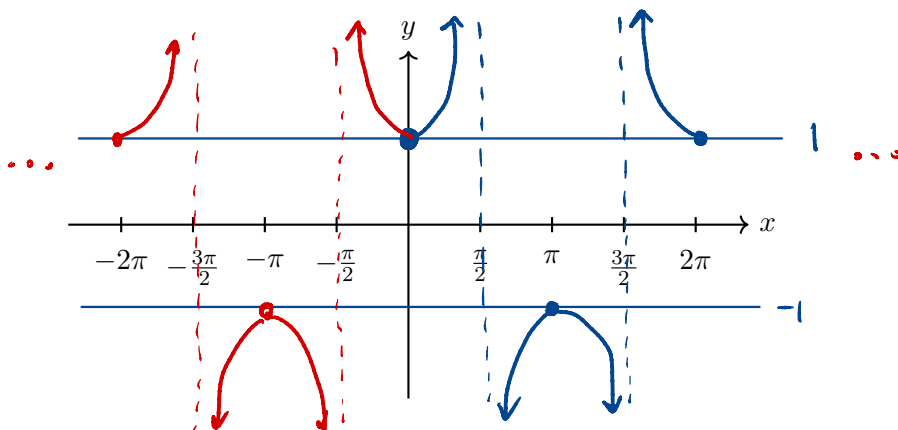
Graph of \sec x
