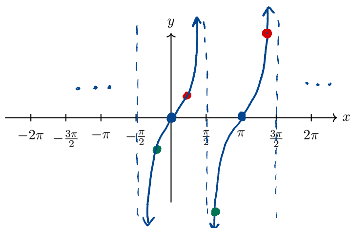
Graph of \tan x
